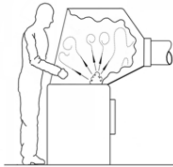
Figure 10.2 - Enclosing Hood
