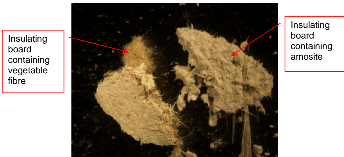
Figure 8.8 – Amosite fibres in asbestos insulating board next to insulating board containing vegetable fibres
